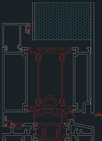
THRESHOLD DETAIL
