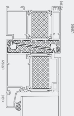
HEAD DETAIL
